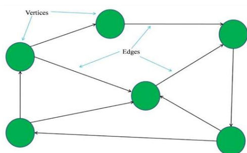
Figure 4. Directed graph.
