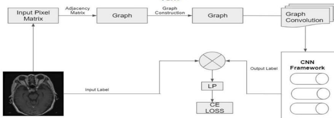
Figure 6. Proposed approach.
