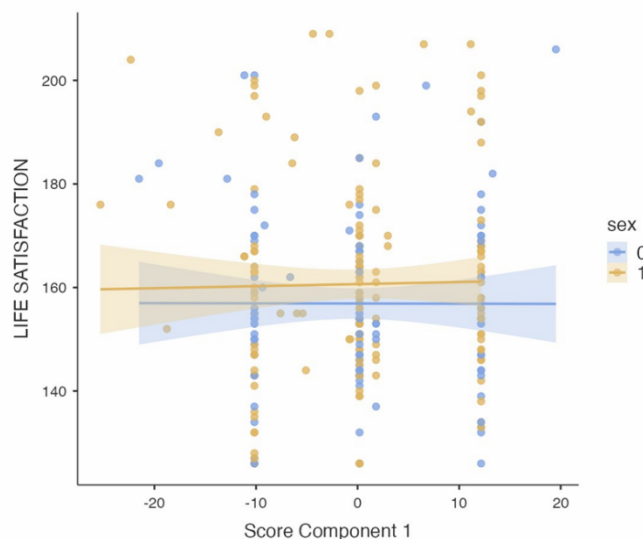
Scatterplot
